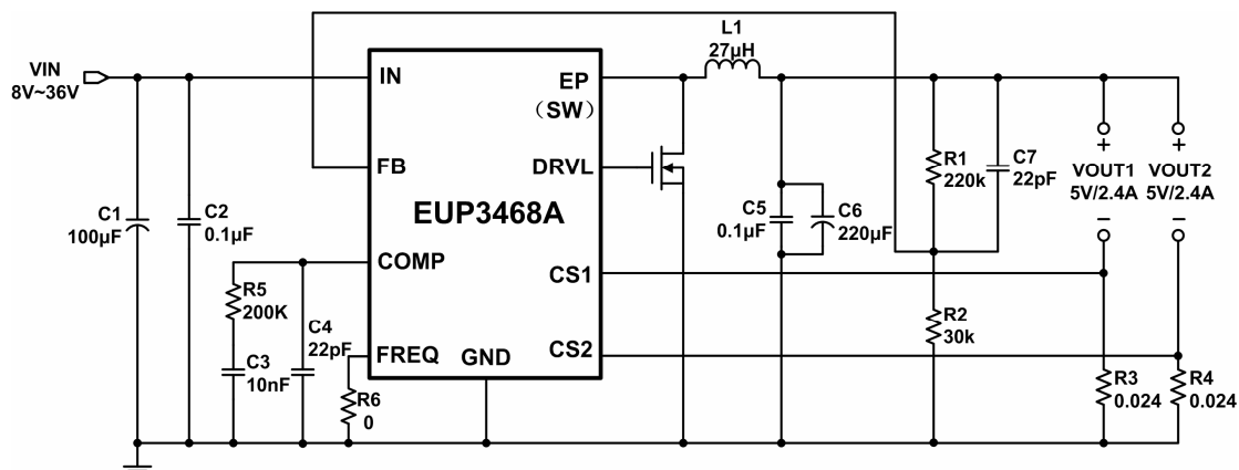
Figure 1. Application Circuit
