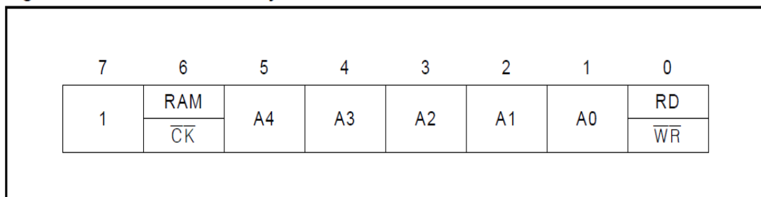
Figure 3. Address/Command Byte
